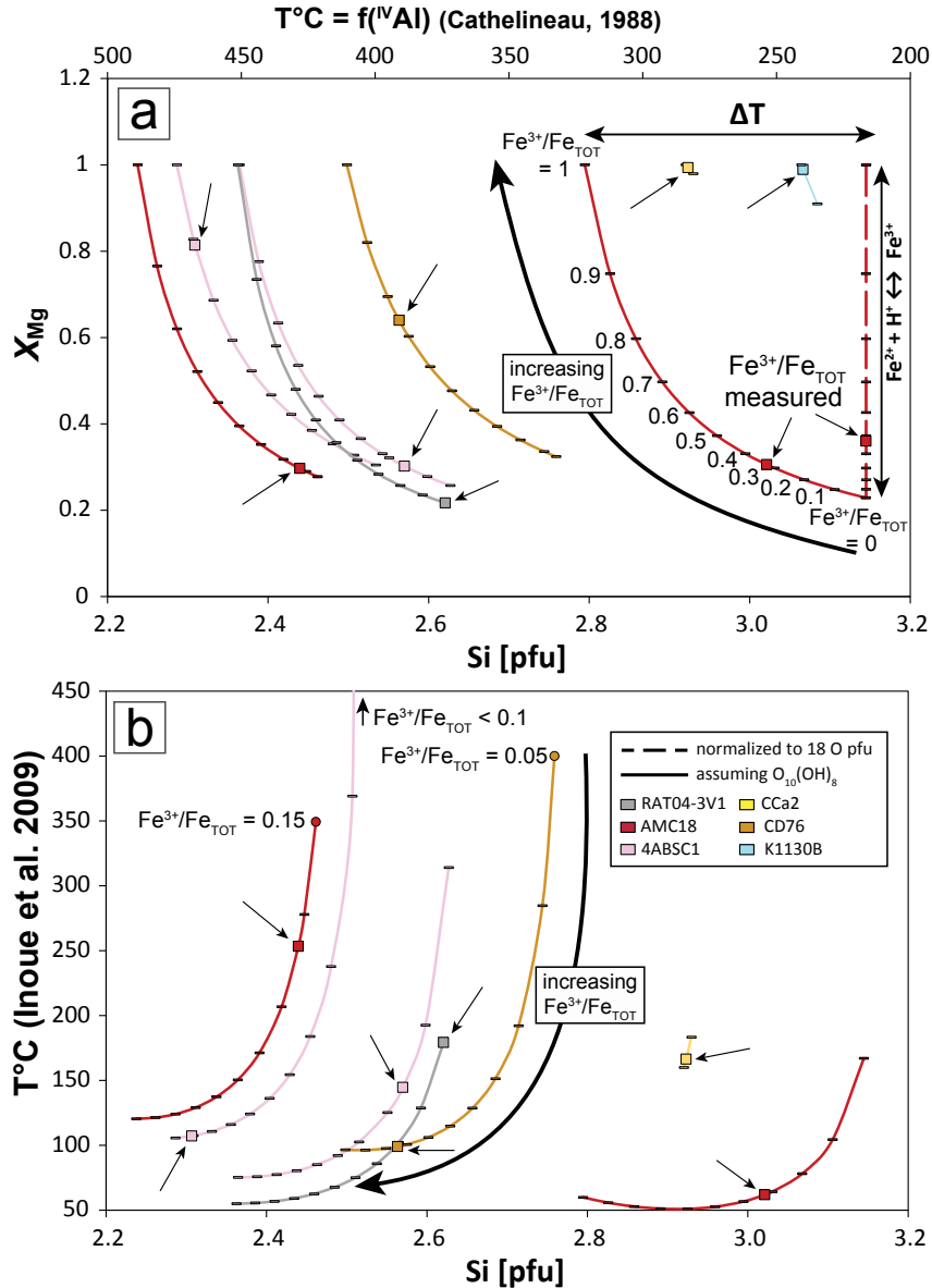
FIGURE 9. Effect of varying \text{Fe}^{3+}/\text{Fe}_{\text{TOT}} on structural formulas and estimated crystallization temperatures for a selection of Fe-poor (CCa2 and K1130B) and Fe-rich chlorite analyses ( \text{Fe}_{\text{TOT}} = total Fe). Solid lines are calculated for the \text{O}_{10}(\text{OH})_8 anionic basis from \text{Fe}^{3+}/\text{Fe}_{\text{TOT}} = 0 (low X_{\text{Mg}} , higher Si content) to \text{Fe}^{3+}/\text{Fe}_{\text{TOT}} = 1 ( X_{\text{Mg}} = 1 , lower Si content). The measured \text{Fe}^{3+}/\text{Fe}_{\text{TOT}} ratio is shown with a square for each chlorite crystal and highlighted with a black arrow. Note that two analyses are plotted for each of the zoned samples 4ABSC1 and AMC18. (a) Evolution of X_{\text{Mg}} and Si content with the temperature estimated using the model of Cathelineau (1988). The vertical dashed line shows the effect of proton loss if the anionic basis is allowed to vary, only for sample AMC18 for readability. The \text{Fe}^{3+}/\text{Fe}_{\text{TOT}} ratio is labeled every 10% for one of the curves; on every other line \text{Fe}^{3+}/\text{Fe}_{\text{TOT}} increases by 10% between black ticks. (b) Evolution of temperature calculated with the model of Inoue et al. (2009) vs. Si content, assuming \text{O}_{10}(\text{OH})_8 anionic basis. Proton loss alters neither Si content nor temperatures estimated with this model. Chlorite from K1130B (sudaite) is not shown in b because its vacancy content is out of the applicability range of the Inoue et al. (2009) model. A similar issue appears with some T estimates for 4ABSC1, where low \text{Fe}^{3+}/\text{Fe}_{\text{TOT}} values cause zero amesite activity and the infinite constant of the reaction.
