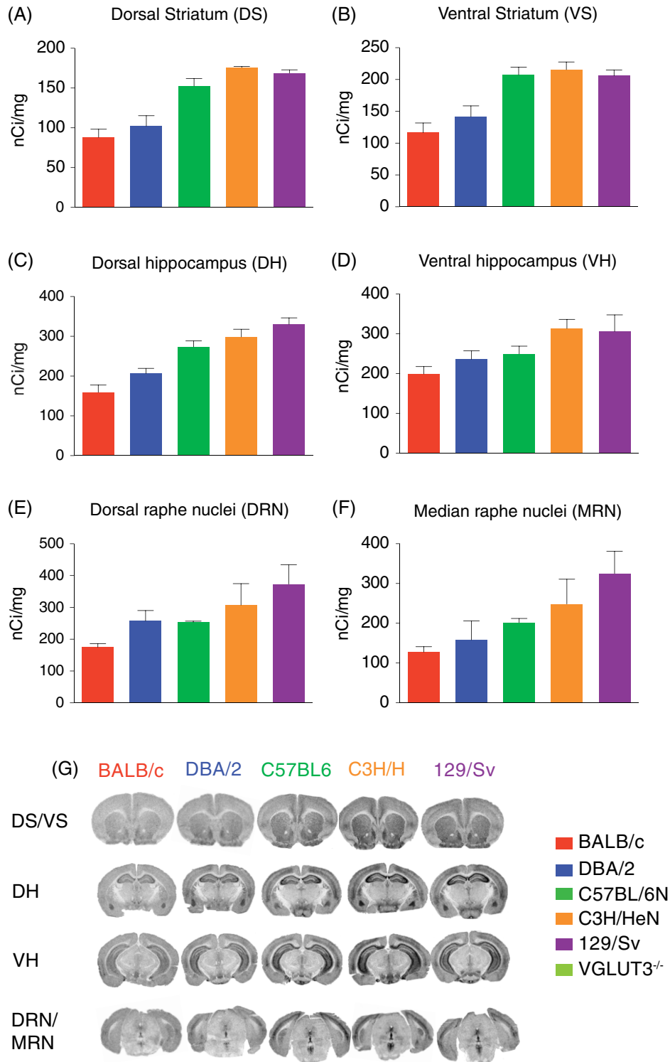
FIGURE 4 Quantification of VGLUT3 content in different brain structures of five mouse lines: (A) DS, (B) VS, (C) DH, (D) VH, (E) DRN, (F) MRN. (G) Representative immunohistochemistry images
