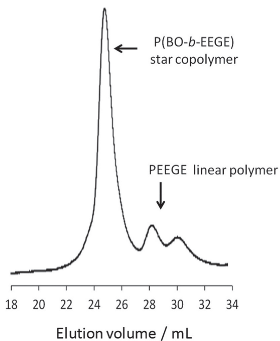
Figure 9. SEC chromatogram of \beta\text{-CD}'\text{-P(BO-}b\text{-EEGE)}_{14} star copolymer (run 6, Table 3) in DMF.
