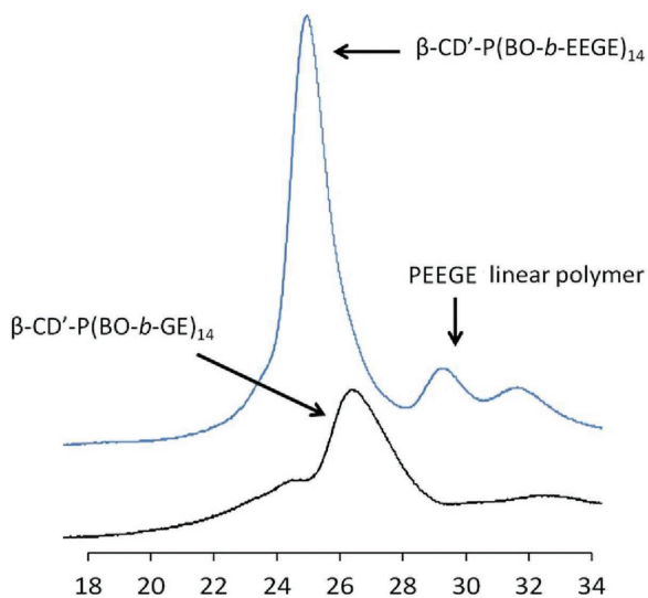
Figure 11. Superposition of SEC chromatograms of \beta\text{-CD}'\text{-P(BO-b-GE)}_{14} and \beta\text{-CD}'\text{-P(BO-b-EEGE)}_{14} .
