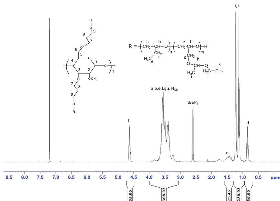
Figure 8. ^1\text{H} NMR spectrum of \beta\text{-CD}'\text{-P(BO-}b\text{-EEGE)}_{14} star copolymer in deuterated chloroform.
