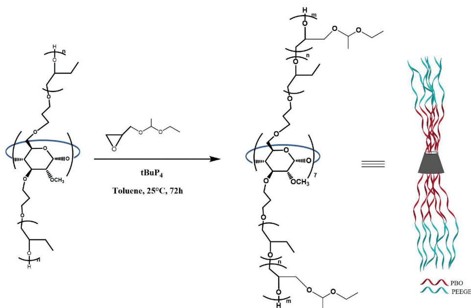
Scheme 4. Pathway route for the synthesis of P(BO- b -EEGE) 14 star copolymer.
