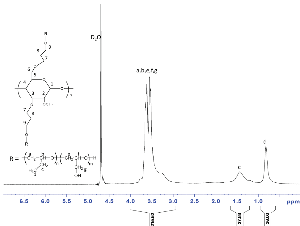
Figure 10. ^1\text{H} NMR spectrum of \beta\text{-CD}'\text{-P(BO-b-GE)}_{14} amphiphilic star copolymer (run 12, Table 4) in deuterium oxide.
