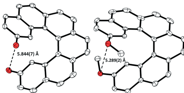
Figure 2. Molecular structures of HELIXOL ( \pm )- 1 (left) and bis(methoxy)helicene ( \pm )- 4 (right) with thermal ellipsoids at 30 % probability.
