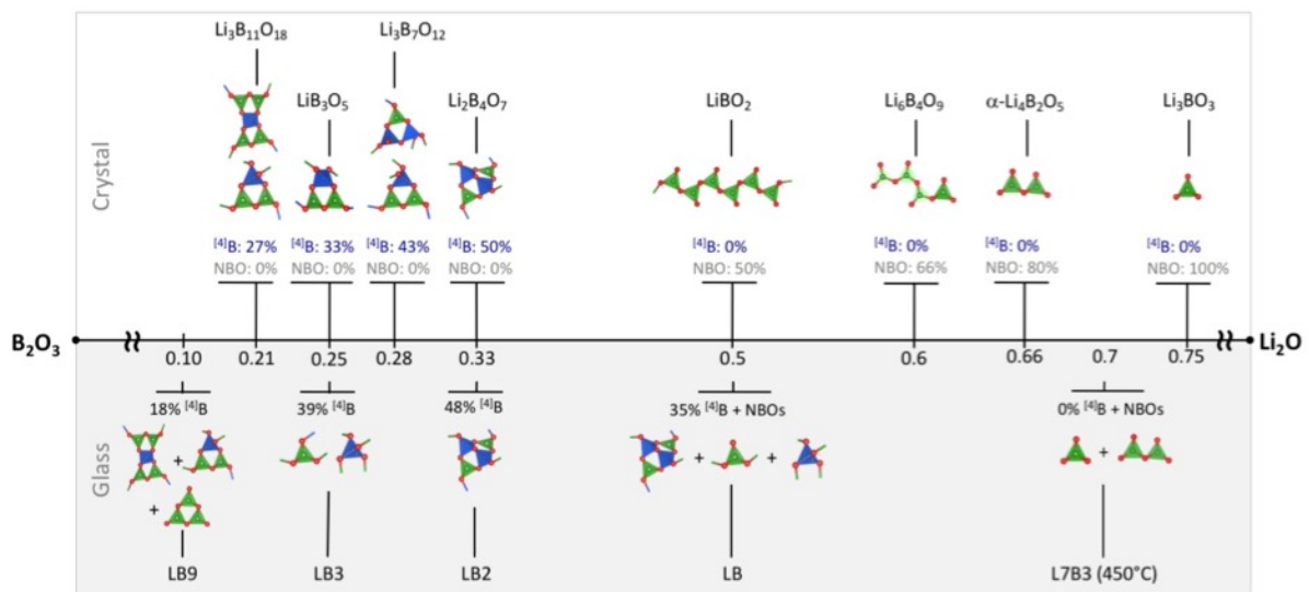
Figure 7: Summary of the superstructural units found in glasses (bottom) and crystalline phases (top) at ambient conditions for the \text{Li}_2\text{O-B}_2\text{O}_3 system.
