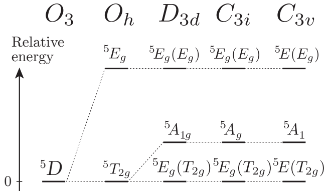
FIG. 3. Lifting of degeneracy of the {}^5D spectroscopic term (free \text{Fe}^{2+} ion) caused by trigonal distortion in the case of siderite.
