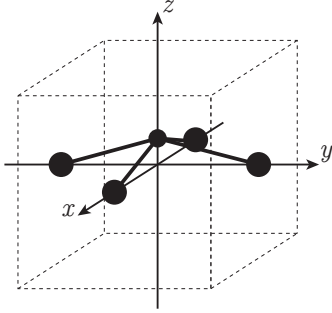
FIG. 8. Orientation for the C_{4v} geometry.
