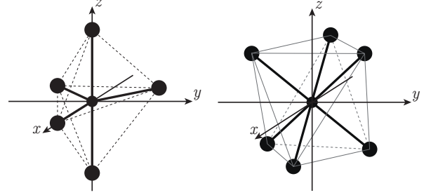
FIG. 7. Orientation of the trigonal bipyramid and the octahedron in C_{3v} .
