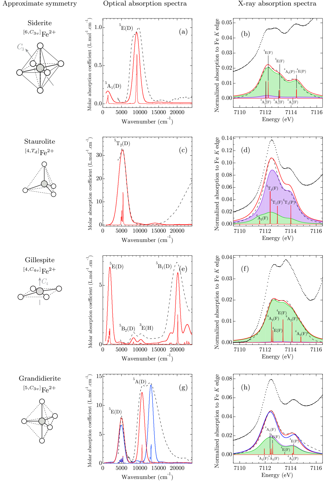
FIG. 2. Optical (left) and X-ray (right) spectra of siderite (a,b), staurolite (c,d), gillespite (e,f), and grandidierite (g,h). The experimental and calculated OAS spectra are in black dashed line (—) and in bold red line (—), respectively. The assignment of the transitions from the ground state is given for each symmetry. The experimental XAS data are in black lines: not corrected ( \cdots ) and corrected (—) from the main edge tail. The calculated XAS K pre-edge spectra are in bold red line (—). Purple and green curves represent the respective contributions of the electric dipole and quadrupole transitions. The assignment of transitions is given using the 3d^7 approximation. For grandidierite, simulated spectra for site A are in red, and spectra for site B are in blue, E1 and E2 XAS features are given for site A only (because they are very similar for site B).
