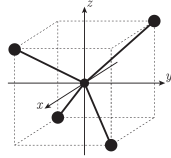
FIG. 6. Orientation of the tetrahedron.
