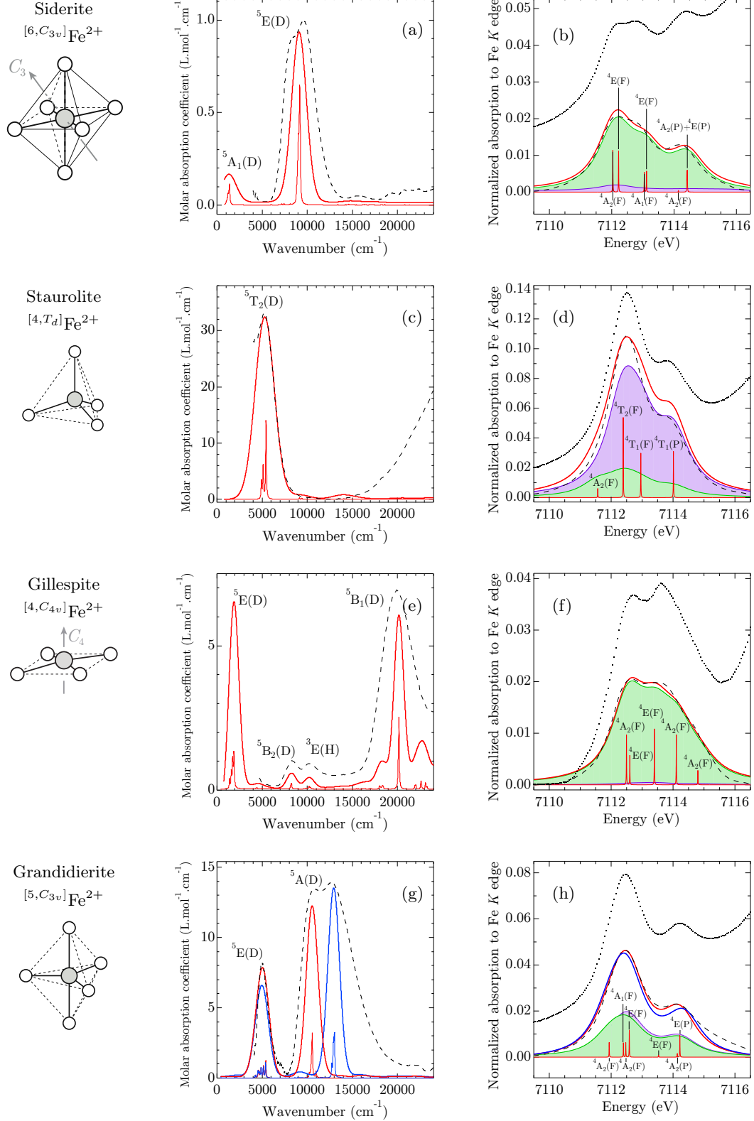
FIG. 2. Optical (left) and X-ray (right) spectra of siderite (a,b), staurolite (c,d), gillespite (e,f), and granddierite (g,h). The experimental and calculated OAS spectra are in black dashed line (—) and in bold red line (—), respectively. The assignment of the transitions from the ground state is given for each symmetry. The experimental XAS data are in black lines: not corrected (···) and corrected (—) from the main edge tail. The calculated XAS K pre-edge spectra are in bold red line (—). Purple and green curves represent the respective contributions of the electric dipole and quadrupole transitions. The assignment of transitions is given using the 3d^7 approximation. For granddierite, simulated spectra for site A are in red, and spectra for site B are in blue, E1 and E2 XAS features are given for site A only (because they are very similar for site B).
