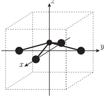
FIG. 8. Orientation for the C_{4v} geometry.
