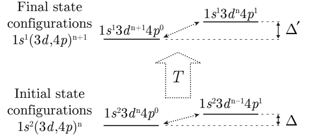
FIG. 1. Configuration interaction used to describe the on-site 4p-3d mixing in the XAS initial and final state configurations. T is the transition operator defined in Eq. (3).
