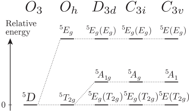
FIG. 3. Lifting of degeneracy of the ^5D spectroscopic term (free Fe^{2+} ion) caused by trigonal distortion in the case of siderite.
