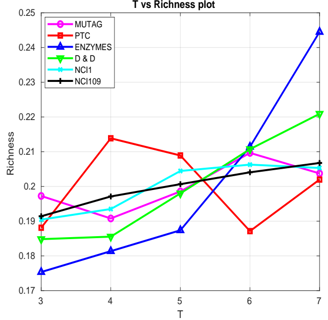
Fig. 1. Richness vs. T plot for MUTAG, PTC, ENZYMES, D & D, NCII and NCII09 datasets.
