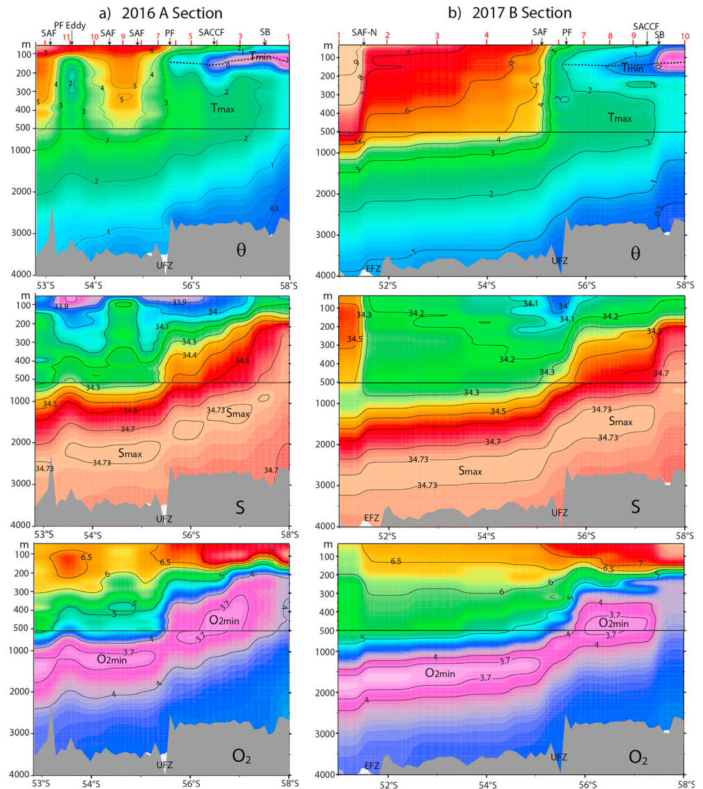
Figure 8. Property sections from (a) the 2016 A section and (b) the 2017 B section. Units are degrees Celsius for potential temperature \theta , unitless Practical Salinity S , and milliliters per liter for oxygen content O_2 . Locations of the hydrography-derived Antarctic Circumpolar Current fronts discussed in the text are indicated beside station numbers (red) on top of the temperature sections. SAF = Subantarctic Front; PF = Polar Front; SACCF = Southern Antarctic Circumpolar Current Front; SB = southern boundary; UFZ = Urdintsev Fracture Zone; SAF-N = northern SAF; EFZ = Eltanin Fracture Zone.
