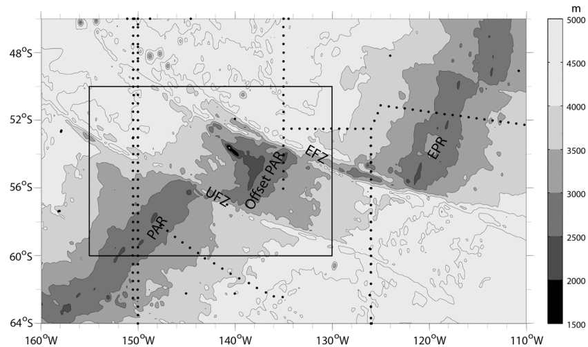
Figure 1. Major bathymetric features and fracture zones in the central South Pacific sector of the Southern Ocean: Pacific Antarctic Ridge (PAR), offset PAR segment, East Pacific Rise (EPR), Udintsev Fracture Zone (UFZ), and Eltanin Fracture Zone (EFZ). The study area (solid rectangle) and historical, high-quality hydrographic sections (dotted lines, http://www.nodc.noaa.gov/OCL/ ) are superposed.
