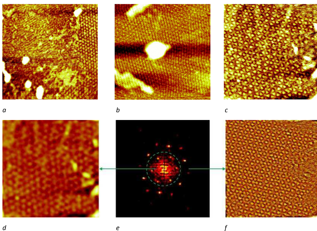
Figure S5: Fourier filtering of the full STM image of Figure 1f: a: full-frame of figure 1e obtained without the top TSB layer. The buried layer was grown with TSB concentration allowing the formation of both dense and honeycomb layers. b: the same as (a) after addition of the top layer, showing various combinations of superposed dense and honeycomb layers. c: full-frame of figure 1f obtained at a low concentration allowing only the formation of honeycomb structures. d-f: Fourier analysis of c. The center image (e) is the Fourier transform (wavevector space), the left image (d) is the low-pass part of c showing triangular molecular network induced by the buried molecules and the right image (f) is the high-pass part of c showing the top honeycomb network (for a given period, the honeycomb network involves higher spatial frequencies than the triangular one). The dashed line circle shows the frontier wavevector amplitude used for filtering.
