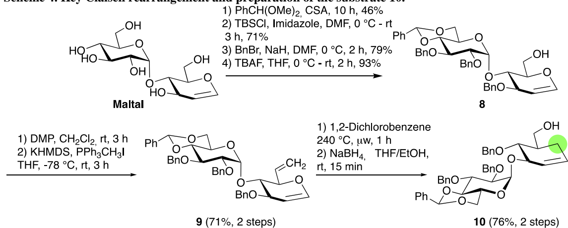
Scheme 5. Synthesis of aziridine carbasugars 4.
