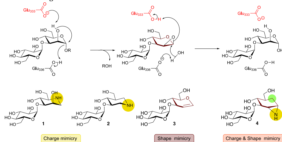
Scheme 1. Postulated enzymatic hydrolytic mechanism for Bacteroides xylanisolvens GH99 (BxGH99), in which catalysis occurs through a 1,2 anhydrosugar intermediate (top). Known, and designed (this work) substrate analogues (below) Residue numbering as in BxGH99.
