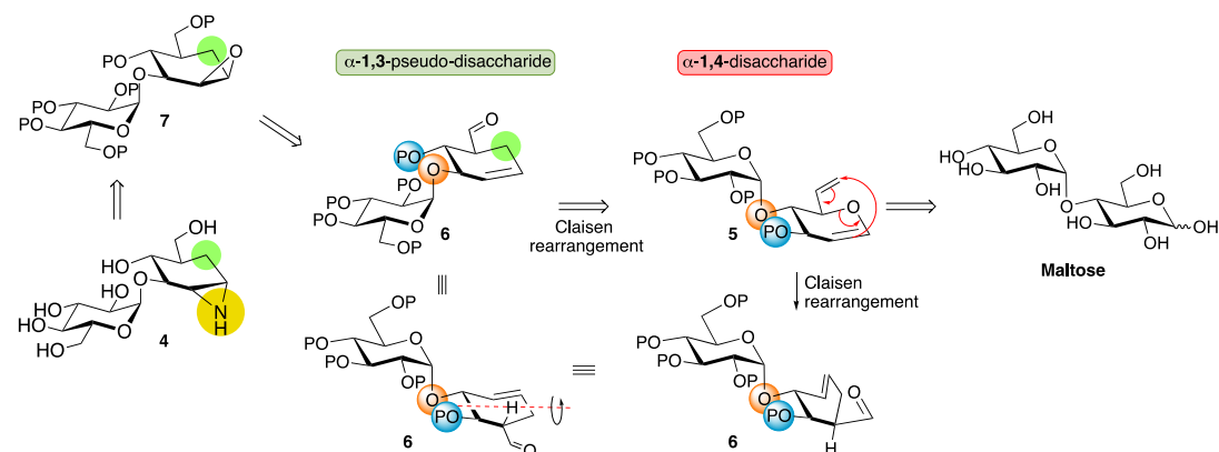
Scheme 3. Retrosynthetic analysis for the synthesis of aziridine 4 .
