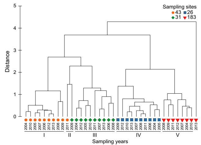
FIGURE 4 Hierarchical cluster analysis (Euclidean distance and average group method) of normalized grain-size fractions ( <30 , 30-63 , 63-250 , 250-500 , 500-2,000 \mu\text{m} ). Symbols indicate sampling sites: 43 (circle), 31 (diamond), 26 (square), and 183 (triangle)
