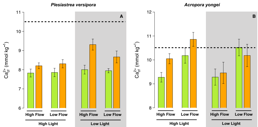
Figure 6. Estimates of the calcium concentration in the calcifying fluid ( \text{Ca}^{2+}_{cf} ) for the corals Plesiastrea versipora and Acropora yongei . \text{Ca}^{2+}_{cf} was calculated from estimates of \Omega_{arag\ cf} and estimates of \text{DIC}_{cf} . Values displayed are mean \pm SE ( n = 6 ). The horizontal dashed line shows the approximate [Ca] in seawater during the experiment. Values displayed are mean \pm SE ( n = 6 ).
