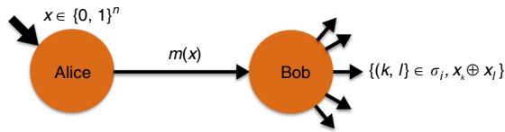
Fig. 1 The Sampling Matching problem. Alice gets an input x \in \{0, 1\}^n and sends a message m(x) to Bob who outputs the pair \langle (k, l) \in \sigma_i, b = x_k \oplus x_l \rangle for a matching \sigma_i , whose distribution is uniform in \mathcal{M} , even conditioned on m(x) . The parity should be correct with high probability for all choices of the matching
