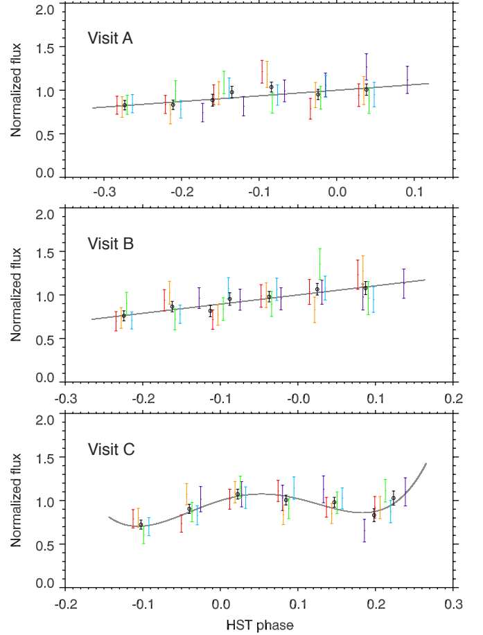
Fig. 3: Lyman- \alpha fluxes for sub-exposures integrated over the entire line and phase-folded on the HST orbital period ( P_{\text{HST}} = 96 min). Phase is between -0.5 and 0.5. Solid grey lines correspond to the best-fit breathing model to the data, which have been scaled to the same nominal flux for the sake of comparison. Black points show sub-exposures binned manually to highlight the breathing trend. Colors correspond to HST consecutive orbits in each visit (orbits 1 to 5 are plotted in purple, blue, green, orange, red).
