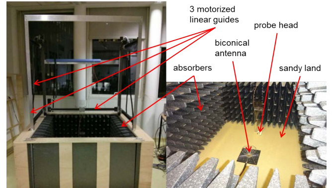
Fig. 4.: Global set-up
