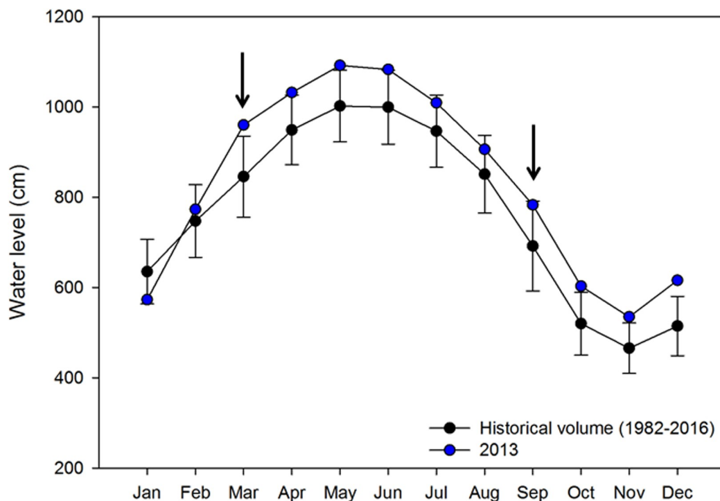
Fig 1. Mean water level and standard deviation in the Lago Grande do Curuai system. Black points indicate historical water level. Blue points indicate water level from the sampling year. Arrows indicate sampling dates. Data source: Agência Nacional de Águas, Hidroweb (data from 1982 to 2016).
