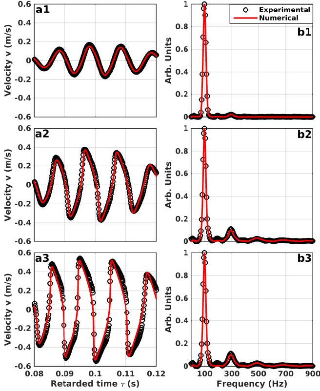
Figure 3. Velocity time waveform (four central periods) at axial position z = 6\text{ cm} (a) and corresponding normalized spectra (b) for shaker excitation amplitude 0.1\text{ m/s} (1), 0.24\text{ m/s} (2) and 0.47\text{ m/s} (3). Measurement (black circles) compared to simulation (red)
