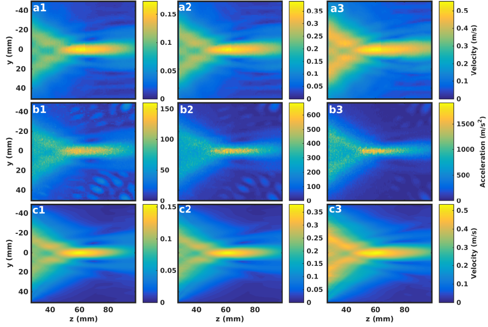
Figure 2. 2D ( y, z ) maps of the measured maximum velocity ( \text{m/s} ) (a) and maximum acceleration ( \text{m/s}^2 ) (b) for shaker excitation amplitudes 0.1m/s(1), 0.24m/s(2) and 0.47m/s(3).
