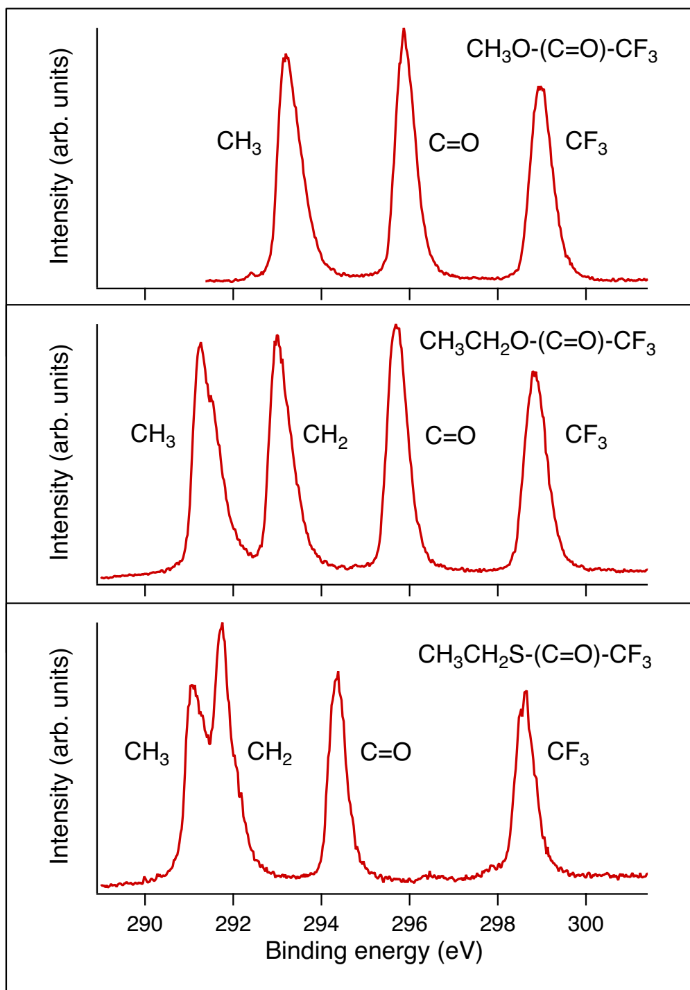
Figure 3: Carbon 1s photoelectron spectra of methyl trifluoroacetate (top), ethyl trifluoroacetate (middle), and S-ethyl trifluoroacetate (bottom). The spectra are recorded at a photon energy of 340 eV. All spectra were recorded at beamline I411 at the MAX II facility in Lund, Sweden.
