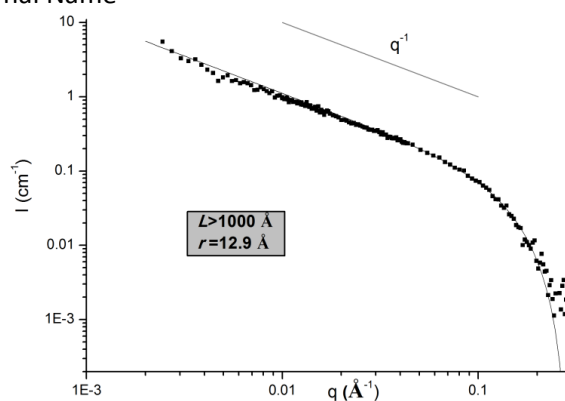
Fig. 3 SANS analysis (●) of ( S )-BTA Trp C12 in C 7 D 8 (5.61 g.cm -3 , 4.4×10 -3 mol.L -1 , 293 K). The curve was fitted (—) according the form factor for rigid rods of infinite length with a circular cross section and a uniform scattering length density ( L =length, r =radius).
