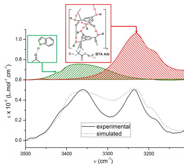
Fig. 2 FT-IR spectrum of (S)-BTA Trp C12 in MCH ( 10^{-2} mol.L -1 , 293 K), zoom on the N-H region (see the C=O region in Fig. S1b). The FT-IR spectra of the models (indole in acetone, 5 \times 10^{-3} mol.L -1 , and BTA Aib in MCH, 10^{-2} mol.L -1 ) are shown with an offset of 600 L.mol -1 .cm -1 . The simulated spectrum is obtained by addition of the FT-IR spectra of indole ( \times 3 ) and of BTA Aib .
