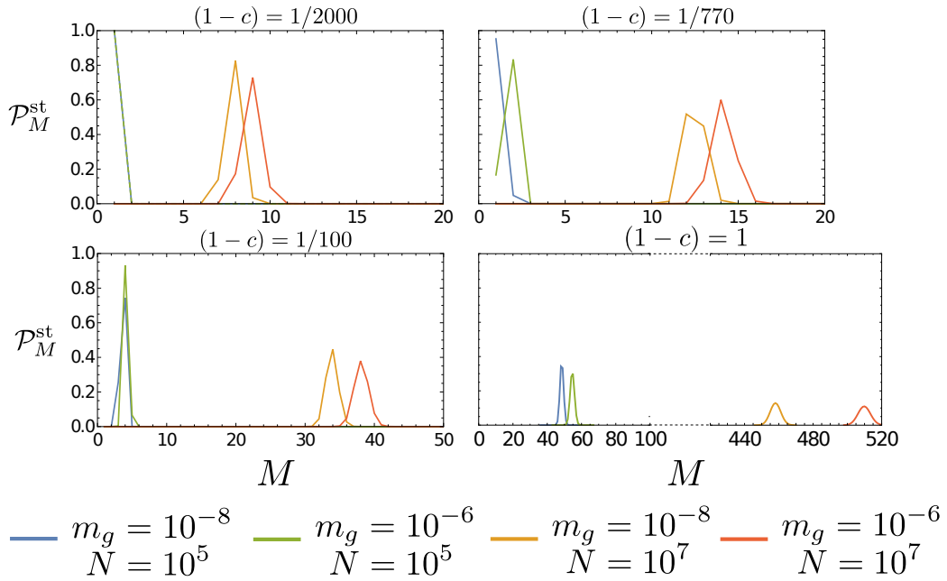
Figure S5: Theoretical distributions for \mathcal{P}_M^{\text{st}} (see Eq. (9) in the Main Text) using parameter values from Table 1 in the Main Text. Panel top-left ( (1-c) = 1/2000 ): parameters estimated for S. cerevisiae . Panel top-right ( (1-c) = 1/770 ): parameters estimated for C. reinhardtii . Panel bottom-left ( (1-c) = 1/100 ): parameters estimated for Tetrahymena. Panel bottom-right ( (1-c) = 1 ): parameters estimated for S. commune . Note that for clarity the scale of the M axis changes between panels. Also note that for the final panel (bottom-right) the region 100 \leq M \leq 400 has been omitted.
