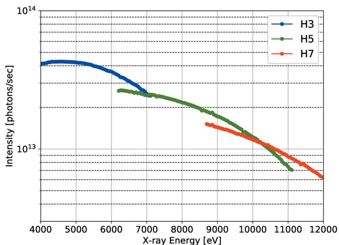
Figure 2 X-ray intensity measured between 4 and 12 keV at the IXS end-station sample position for the third (H3), fifth (H5) and seventh (H7) undulator harmonics at a ring current of 430 mA, using the silicon (111) DCM and the M2B focusing mode. In the KB focusing mode, the X-ray intensity is a factor of three less than these values (see Section 1.1).
