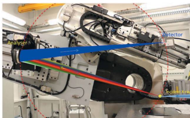
Figure 4 Photograph of the IXS single-analyser spectrometer superimposed with the Rowland circle geometry (represented by the dashed red circle). Monochromatic X-rays are focused at the sample and the scattered and fluorescence X-rays are collected by the analyser crystal that selects a narrow energy band of these X-rays which are then focused at the detector position. The spectrometer energy is scanned by varying the Bragg angle of the analyser whilst maintaining the Rowland circle geometry. Note that a helium flight path, which reduces the effect of air absorption, is omitted from the photograph for clarity.
