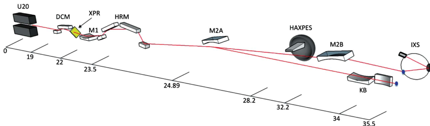
Figure 1 Side-view schematic of the optical layout for the IXS end-station. Beam propagation is from left to right and distances are in metres from the centre of the U20 undulator. Beamline apertures and X-ray beam diagnostics such as beam-position monitors and imagers are not shown for clarity. Refer to the main text for details on the abbreviations used.
