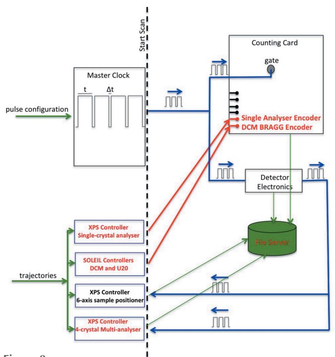
Figure 8 Control system schematic for GALAXIES on-the-fly scanning. These continuous scans are used for scanning both the incident (DCM and undulator) spectrometer energies and also the sample position. The master clock is used to gate the counting card and trigger the detector electronics and Newport XPS controllers. See main text for a more detailed explanation of the system.
