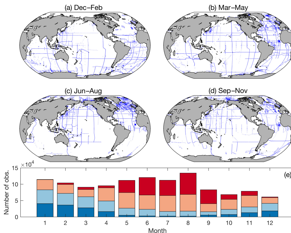
Figure 7. Distribution of data in GLODAPv2.2019 in (a) December–February, (b) March–May, (c) June–August, and (d) September–November and (e) number of observations for each month north of 45^\circ N (red), north of the Equator to 45^\circ N (orange), the Equator to 45^\circ S (light blue), and south of 45^\circ S (dark blue).
