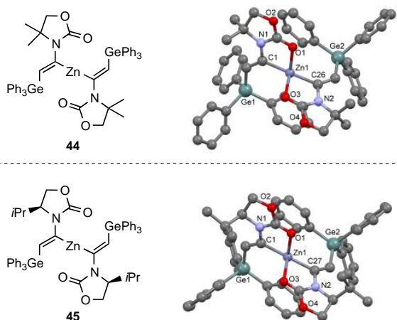
Figure 1. X-ray crystal structure of 44 and 45 . Selected bond lengths and bond angles. 44 : \text{Zn}\text{-C}1 = 1.995(8) Å, \text{Zn}\text{-C}26 = 1.985(8) Å, \text{C}1\text{-Zn}\text{-C}26 = 170.8(3)^\circ , \text{O}1\text{-Zn}\text{-O}3 = 97.8(3)^\circ . 45 : \text{Zn}\text{-C}1 = 1.989(7) Å, \text{Zn}\text{-C}27 = 2.009(7) Å, \text{C}1\text{-Zn}\text{-C}27 = 165.5(3)^\circ , \text{O}1\text{-Zn}\text{-O}3 = 91.3(3)^\circ .
