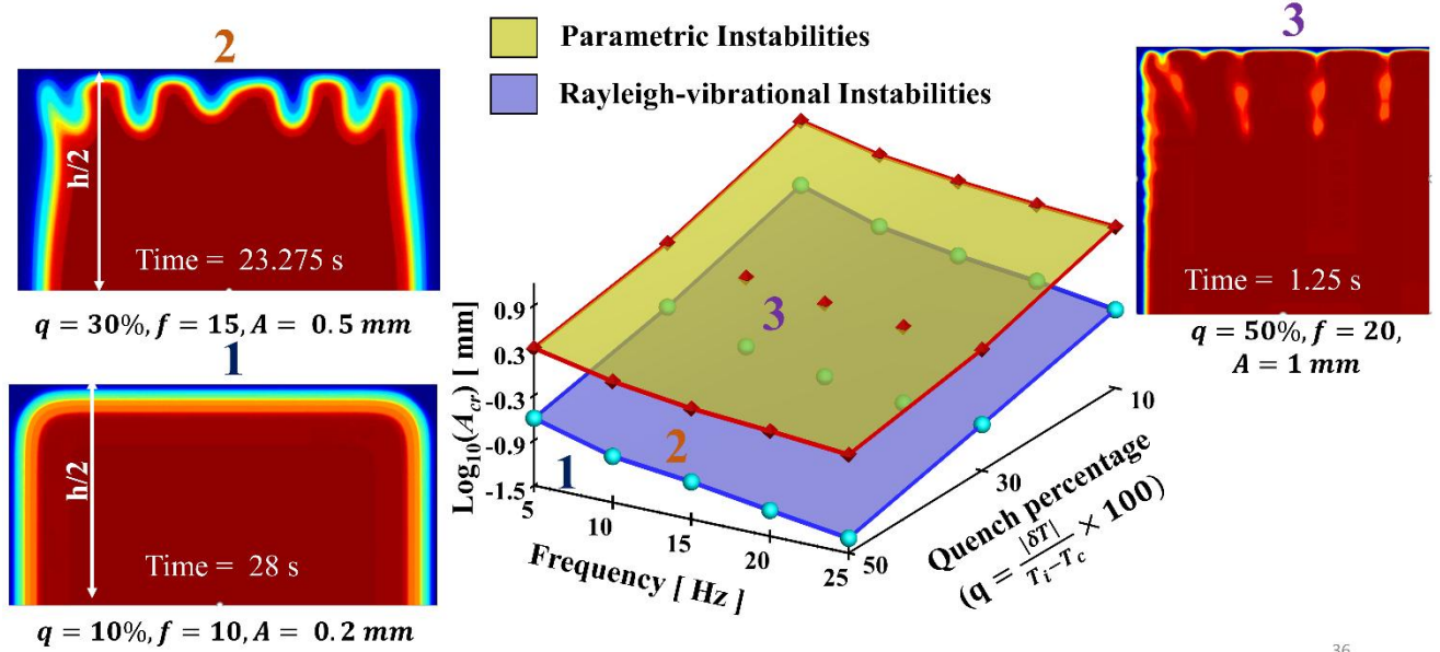
Figure 18. Stability plot illustrating different instabilities based on their operating conditions for T_i - T_c = 500 \text{ mK} .
