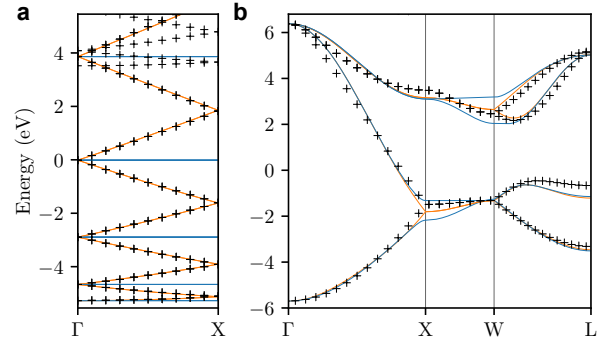
FIG. 5: Comparison between the bands obtained using the earlier interpolation procedure (blue lines), those obtained using the (current) modified approach of Eq. (47) (orange lines), and the ab initio bands (black crosses). (a) Linear chain of carbon atoms, with 12 atoms per unit cell (separated by a distance of 1.3 \text{ \AA} along the z direction) and \Gamma -point sampling. 36 Wannier functions have been computed starting from projections over p_x and p_y orbitals on carbon atoms and s -orbitals midbond between them. A frozen window up to the Fermi energy (set to zero in the plot) has been considered, while the disentanglement window included all states up to \sim 14 \text{ eV} above the Fermi level. (b) Bulk silicon, with the BZ sampled on an unconverged 3 \times 3 \times 3 grid of k -points.
