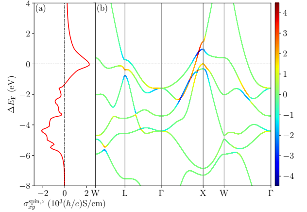
FIG. 6: (a) Intrinsic spin Hall conductivity \sigma_{xy}^{\text{spin},z} of fcc Pt, plotted as a function of the shift in Fermi energy relative to its self-consistent value. (b) Band structure of fcc Pt, colour-coded by a dimensionless function r(\Omega_{nk,xy}^{\text{spin},z}) of the spin Berry curvature [Eq. (57b)]. The function r(x) is equal to x/10 when |x| < 10 , and to \log_{10}(|x|)\text{sgn}(x) when |x| \geq 10 .
