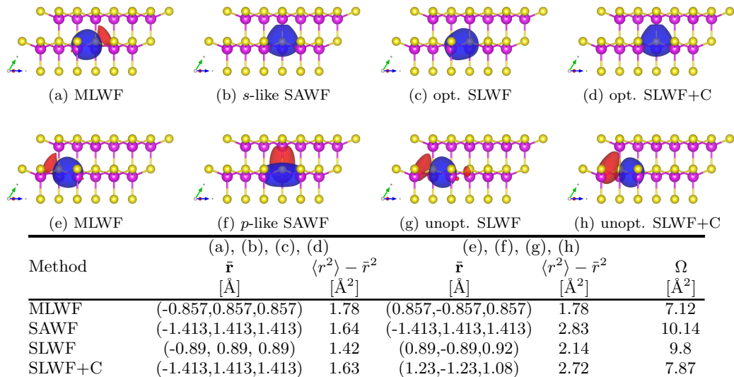
FIG. 1: Top (figure): comparison of two Wannier functions representatives resulting from different minimisation schemes for gallium arsenide (larger pink spheres: Ga cation atoms, smaller yellow spheres: As anions): (a), (e) MLWF; (b), (f) SAWF; (c), (g) SLWF; (d), (h) SLWF+C. For MLWF, SLWF and SLWF+C, four s -type orbitals centred at the midpoints of the four Ga–As bonds ((1/8, 1/8, 1/8), (1/8, 1/8, -3/8), (-3/8, 1/8, 1/8), (1/8, -3/8, 1/8)) were used as initial guess. In the case of SLWF and SLWF+C, we optimise the first WF (and also constrain its centre to sit at (1/4, 1/4, 1/4) , i.e. on the As atom, for SLWF+C), while all the other WFs are left unoptimised. For SAWF, one s -type and three p -type orbitals centred on the As atom are used as initial guess. Specifically, the first row shows one MLWF (a), one SAWF with s character centred on As (b), one WF obtained with the selective localisation scheme (c) and one WF obtained with the selective localisation scheme with additional constraints on its centre (d). The second row shows one of the other three WFs for all four methods. In particular: (e) MLWF, (f) SAWF with p character, (g) unoptimised SAWF and (h) unoptimised SAWF+C. For all plots we choose an isosurface level of \pm 0.5 \text{ \AA}^{-3/2} (blue for + values and red for - values) using the Vesta visualisation program 28 . Bottom (table): Cartesian coordinates of the centres \bar{\mathbf{r}} and minimised individual spreads \langle r^2 \rangle - \bar{r}^2 for the two representative Wannier functions of each of the four different minimisation schemes and initial guesses described above. We also report the total spread \Omega of all four valence WFs for each method.
