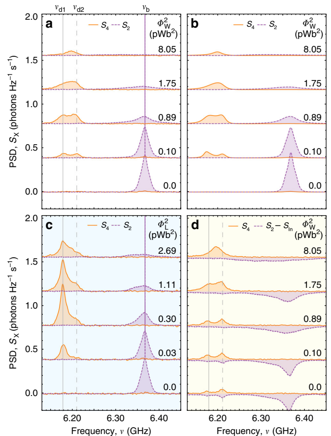
Fig. 3 Measured power spectral densities (PSD). PSD of radiation extracted from the resonator S_4(\omega) (solid orange lines) and re-emitted into the transmission line S_2(\omega) (dashed purple lines) for coherent excitation as a function of a white noise power \Phi_W^2 and c Lorentzian noise power \Phi_L^2 . b Master equation calculations of S_4(\omega) and S_2(\omega) for coherent excitation as a function of \Phi_W^2 . d Measured PSD for incoherent excitation as a function of \Phi_W^2 . Dashed purple lines represent a difference between measured S_2(\omega) and PSD of incoherent microwave radiation S_{\text{in}} . PSD for different noise powers are displaced by 0.2 \text{ photons s}^{-1} \text{ Hz}^{-1}
