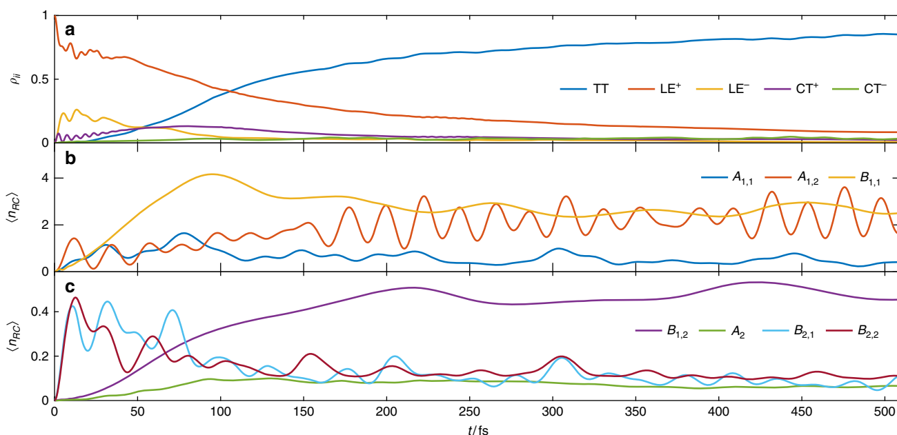
Fig. 4 Simulated SF dynamics in DP-Mes. Electronic populations ( a ) and environmental RC occupation dynamics ( b , c ). For <20 fs, damped Rabi oscillations transfer the population from LE^+ to LE^- and CT^+ . At subsequent times TT mirrors the LE^+ decay leading to SF on a time scale of 200 fs and suggesting a direct SF pathway. Similar time scales are present in the bath excitation n_{RC} of B_1 and B_2 . The final TT yield reaches 90% after 1 ps
