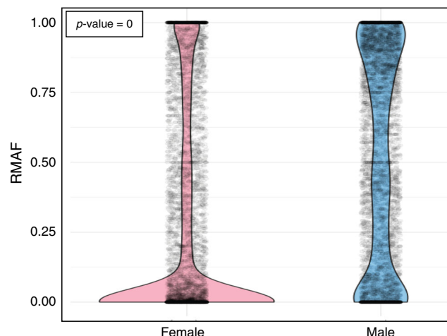
Fig. 3 RNA-mutated allele frequency (RMAF) for X-chromosome genes was particularly high in male cancers, while in female cancers most mutations were not expressed. RMAF was calculated for the 12 disparity cancers, for females and males independently (and pertinently this combined data reflects the individual cancers as evident in Supplementary Fig. 2c). RMAF was quantified using a scale between 0 and 1. For a specific exome nucleotide mutation, 0 indicates the complete absence of mRNA for this particular mutation, where the gene is expressed at the mRNA level; 1 defines mutation in this nucleotide in the corresponding mRNA in 100% of cases. Females are indicated in pink and males in blue.
