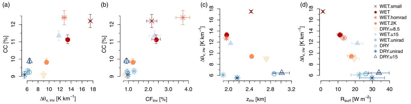
FIGURE 8 Scatterplots of cloud cover as a function of (a) inversion strength and (b) inversion cloudiness (defined as the cloud fraction maximum within 400 m below the inversion height), and inversion strength as a function of (c) inversion height and (d) surface rain rate. The symbols represent the mean and the whiskers represent the standard error ( \pm\sigma/n , where n represents number of independent samples [every 4 h]) in the near-equilibrium regime of the simulations (see Table 1 for the averaging periods of individual simulations)
