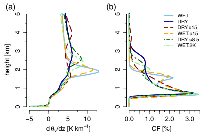
FIGURE 1 Domain-averaged profiles of (a) stability and (b) cloud fraction for the WET , the DRY , the DRY.u15 , the WET.u15 , the DRY.ω8.5 , and the WET.2K simulations
