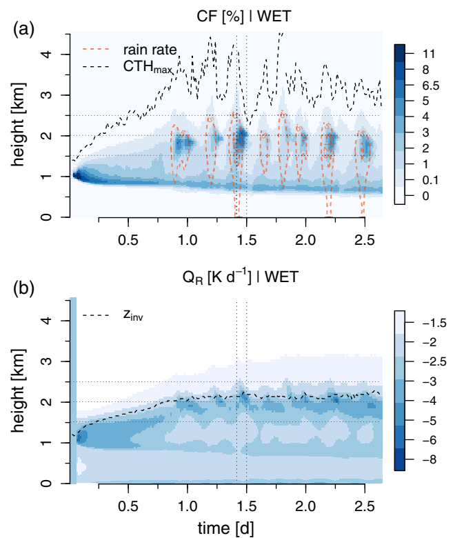
FIGURE 2 Temporal evolution of domain-averaged profiles of (a) cloud fraction and (b) radiative heating tendency Q_R for the WET case. The contour lines in (a) represent the precipitation amount in intervals of 5, 12.5 and 20 mg·kg -1 . Furthermore, the maximum cloud-top height and the inversion height are indicated in (a) and (b), respectively. Horizontal and vertical reference lines are added to facilitate the comparison of different features
