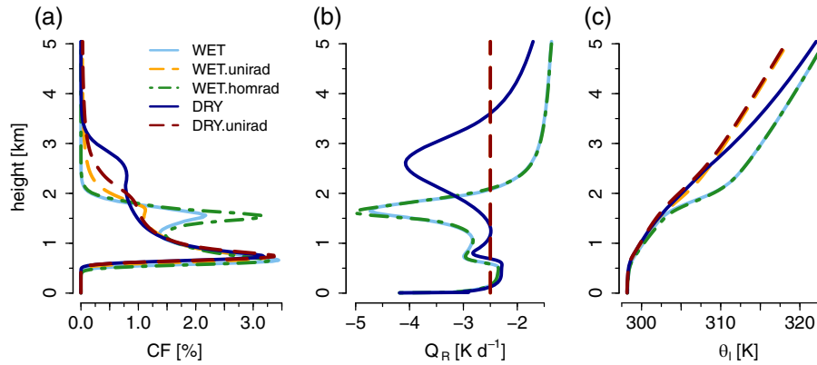
FIGURE 5 Domain-averaged profiles of (a) cloud fraction, (b) radiative heating tendency, and (c) liquid water potential temperature, for the WET, the WET.unirad, the WET.homrad, the DRY, and the DRY.unirad simulations
