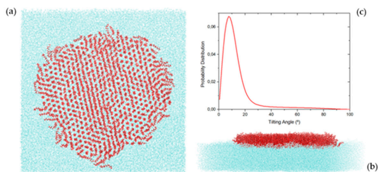
Figure 7. Snapshots of a simulation of 550 C_{11}F_{23}CO_2H molecules monolayer at the surface of the water at 0.6 \text{ nm}^2/\text{molecule} and 298 K; (a) top-view; (b) side-view; (c) tilt angle distribution.
