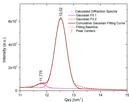
Figure 8. Calculated diffraction spectrum computed from molecular dynamics (MD) simulation of C_{11}F_{23}CO_2H monolayer at 298.15 K of Figure 7.
