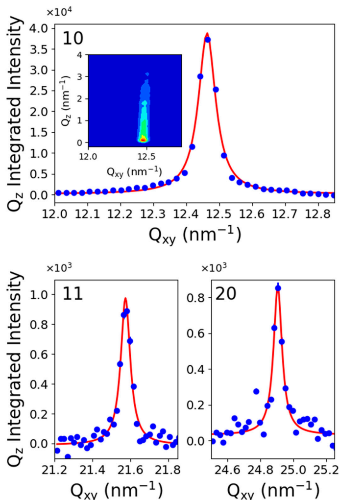
Figure 6. Diffraction spectra of C_{11}F_{23}CO_2H at 18\text{ }^\circ\text{C} and 15\text{ mN/m} . Top: (10) peak; Bottom (11) and (20) peaks.
