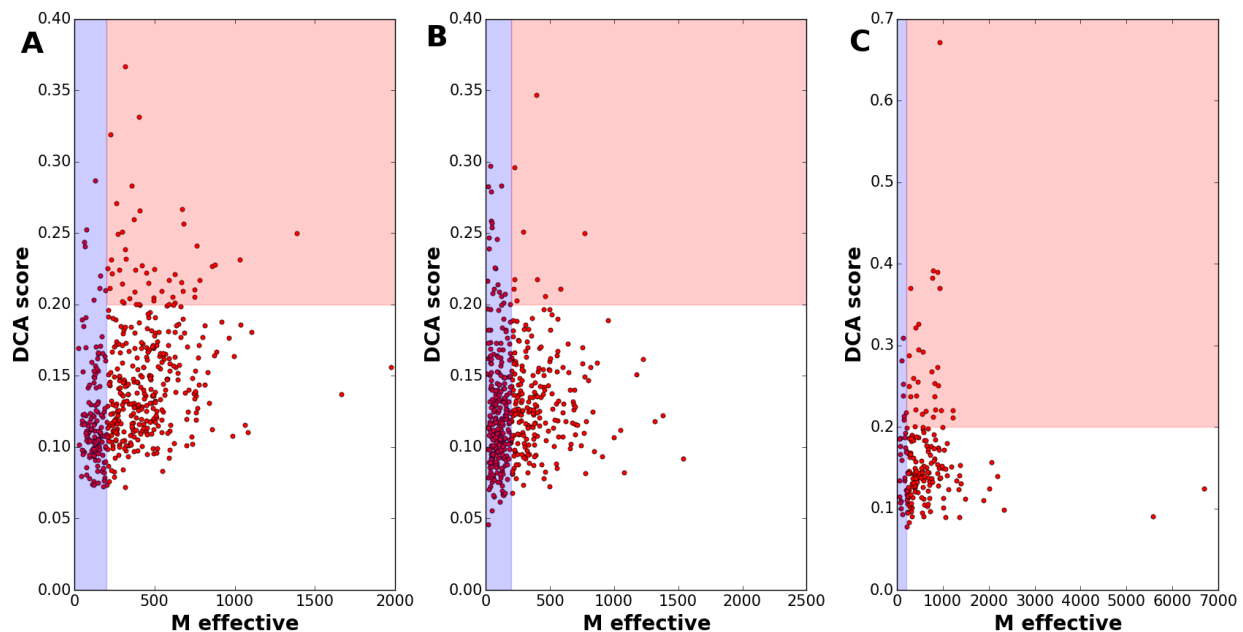
Figure 4: DCA identifies strong residue-scale coevolution between phyletically coupled domain pairs – Panel A shows the effective sequence number (defined as the sequence number at 80% maximum sequence identity, cf. Supplement for the precise definition) and the DCA scores for the 500 domain pairs of strongest phyletic coupling not belonging to the positive-relation set (i.e. the 500 most
