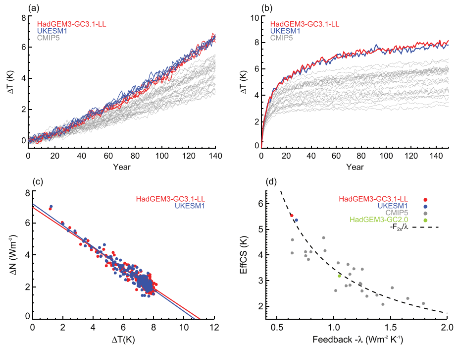
Figure 1. Global annual mean surface air temperature change ( \Delta T ) in the (a) 1pct\text{CO}_2 and (b) abrupt-4x\text{CO}_2 simulations. (c) Gregory plot used to estimate the EffCS. (d) Relationship between EffCS and feedback parameter ( \text{EffCS} = -F_{2x}/\lambda ); the dotted line uses the CMIP5 multimodel mean \text{Eff}F_{2x} .
