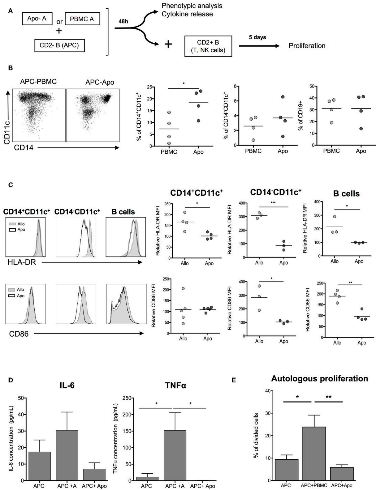
FIGURE 4 | Apoptotic cells induce hyporesponse of allogeneic cells: indirect presentation pathway. (A) Experimental scheme. APCs (CD2– cells) were incubated with allogeneic Apo-cells or untreated irradiated-allogeneic PBMCs for 48 h. Phenotypic analysis was done on APCs, which were then used to stimulate autologous, CFSE-stained CD2+ cells. (B) Flow cytometry analysis of APCs showing the ratio of CD14+CD11c–, CD14+CD11c+, and CD19+ cells. (C) Left: overlay comparison (Continued)
