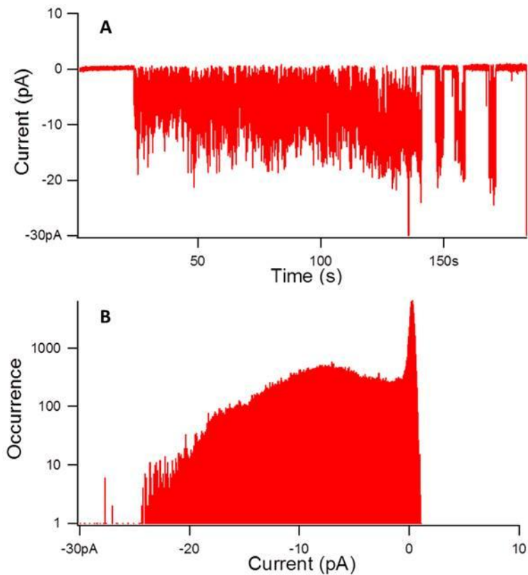
Figure 6. BLM results for TBCP3 at 10 \mu\text{g.mL}^{-1} , for an applied voltage of -100 \text{ mV} , in 1 \text{ M KCl} , 5 \text{ mM HEPES} , \text{pH}=7.4 , at room temperature (A) Current as a function of time. (B) Occurrence as a function of current (current distribution).
