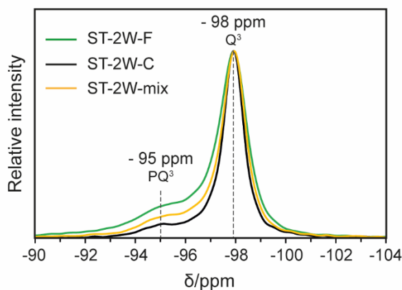
Figure 11. 29 Si MAS-NMR spectra of the fine and coarse fractions of a synthetic talc of two weeks of synthesis.
