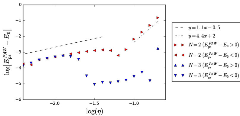
FIGURE 3. Error on the lowest eigenvalue of the PAW equations with pseudopotentials including odd PAW functions.
