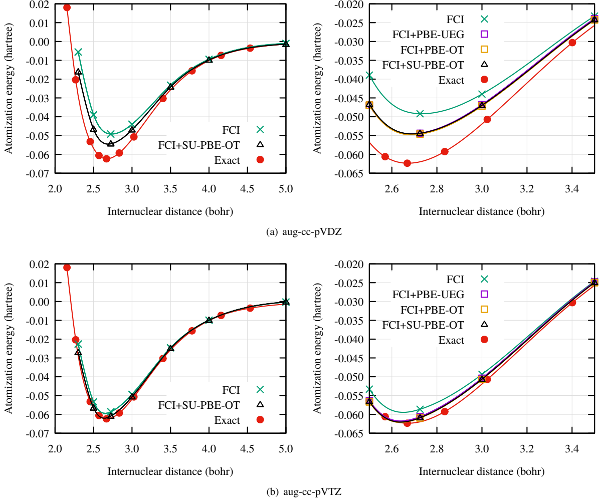
FIG. 4. Potential energy curves of the F_2 molecule calculated with exFCI and basis-set corrected exFCI using the aug-cc-pVDZ (top) and aug-cc-pVTZ (bottom) basis sets. The estimated exact energies are based on a fit of experimental data and obtained from Ref. 87.
