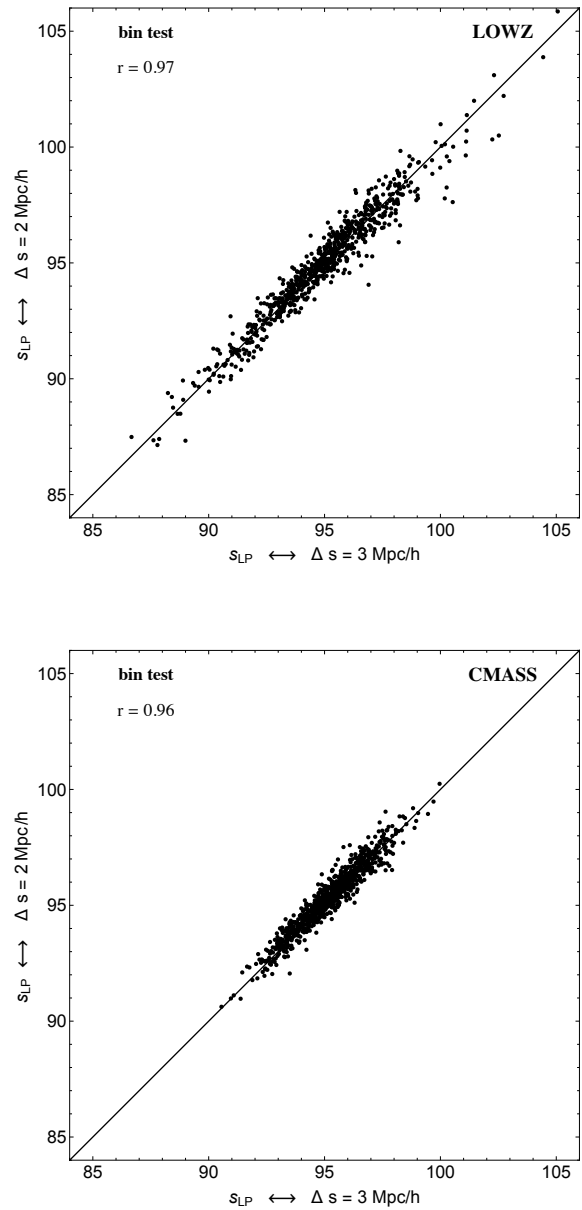
FIG. 5: LP-estimator scatter plot, for a quintic-polynomial fit to the CF, with bins of width \Delta s = 2 and 3 Mpc/h, for the LOWZ ( upper panel ) and CMASS ( lower panel ) mock catalogues.
