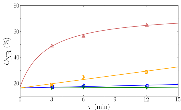
Fig. 4 Percentage of Nile red measured on a ATBC solution located on top of an emulsion when incubated ( \nabla ), i.e. non-insonified, or insonified at a pressure of 0.4, 3.5 or 7 MPa ( \blacktriangleleft , \blacktriangleright and \blacktriangle respectively) during a time \tau of 3, 6, or 12 min. For P_{pkpk} < 7 MPa, a linear fit led to a slope of 0.04, 0.20, and 1.11 for 0, 0.4 and 3.5 MPa, respectively. All fit curves start at approximately 16.6% at t = 0 .
