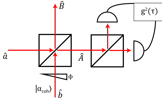
Figure 1. Schematic setup for the creation of anti-bunched states. The two input operators are indicated by \hat{a} and \hat{b} , and the corresponding output operators are denoted by \hat{A} and \hat{B} . The input mode \hat{b} consists of a coherent state with a tunable phase \phi relative to \hat{a} . Several input states \hat{A} are studied in this paper. The correlation function is computed on the output mode \hat{A} in the same way as is done experimentally, i.e. using a beamsplitter and two photodetectors as represented.
