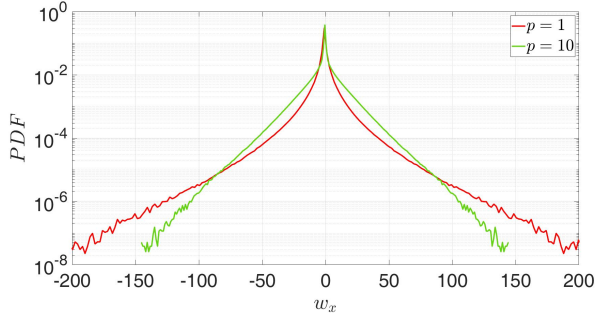
FIG. 9. Probability distribution function of the vorticity along the x -direction at the peak of the energy dissipation for the runs at resolution 1024^3 for p = 1 and p = 10 . The distributions were computed inside the impermeable box, with the same conditions as in Fig. 8.
