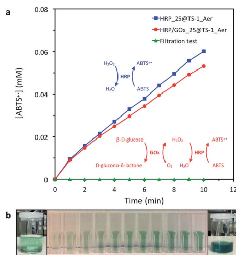
Fig. 6 Colorimetric assay of HRP using ABTS as substrate. (a) Kinetic data for the formation of ABTS •+ catalyzed by HRP in HRP 25 @TS-1_Aer and HRP/GOx 25 @TS-1_Aer. Filtration tests proved that the enzymatic activity was located in the solid (see one example for HRP/GOx 25 @TS-1_Aer in the figure, see also Fig. S6†). (b) Evolution of the color of the solution as a function of the production of ABTS •+ catalyzed by HRP in HRP 25 @TS-1_Aer. Experimental conditions: 10 mM citric acid-phosphate pH 6.0, tests carried out at room temperature ( ca. 23 °C). The detailed experimental procedures are presented in the ESI.†
