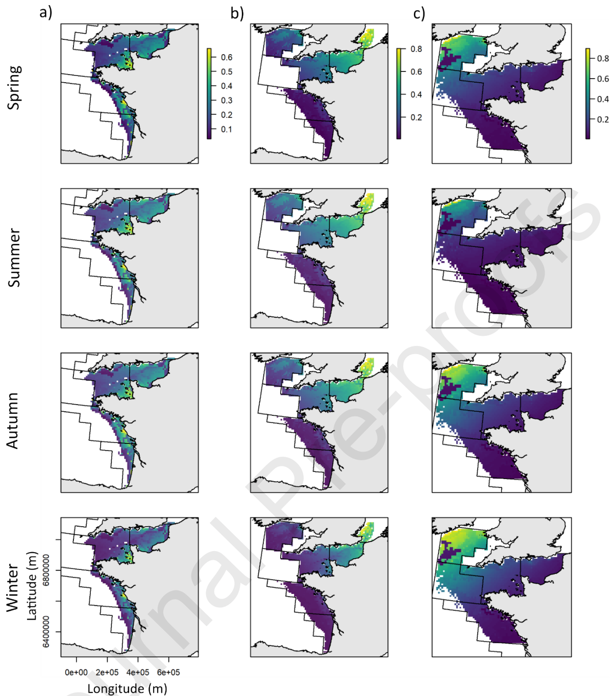
Fig. 2. a) Raja undulata b) Raja clavata and c) Raja montagui prediction maps (10 km 2 cells) per season (three month period). The legend represents the probability of presence. Black solid lines delineate ICES statistical divisions.
