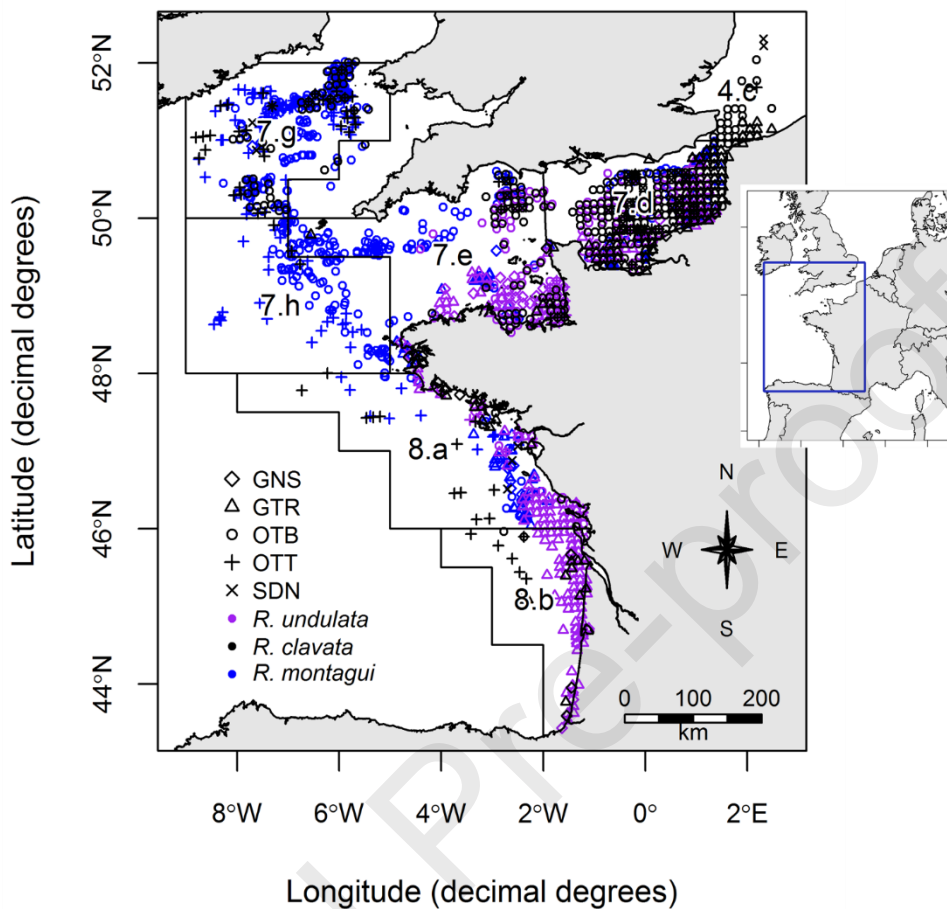
Fig. 1. Location of the study area with fishing vessel presence hauls of Raja undulata (purple), Raja clavata (black) and Raja montagui (blue) between 2009 and 2017. The different colour points represent the different gear types: set gillnets (GNS, \diamond ), trammel nets (GTR, \triangle ), otter beam trawls (OTB, \circ ), otter twin trawls (OTT, + ) and Danish seine nets (SDN, \times ). Black solid lines delineate ICES statistical divisions and their coded name.
