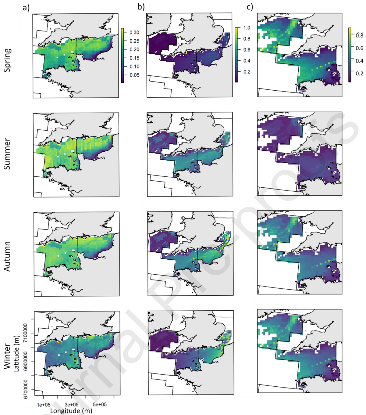
Fig. 4. Mature a) Raja undulata b) Raja clavata c) Raja montagui predicted distribution maps (10 km 2 cells) per season (three month period). The legend represents the probability of presence. Black solid lines delineate ICES statistical divisions.
