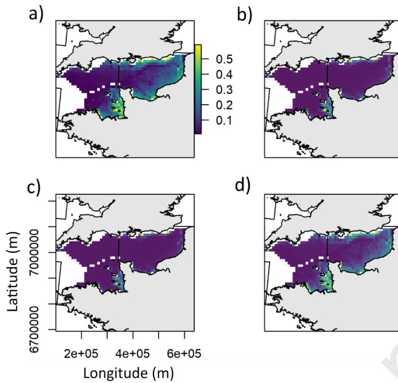
Fig. 3. Juvenile Raja undulata predicted distribution maps (10 km 2 cells) per season a) spring b) summer c) autumn and d) winter. The legend represents the probability of presence. Black solid lines delineate ICES statistical divisions.
