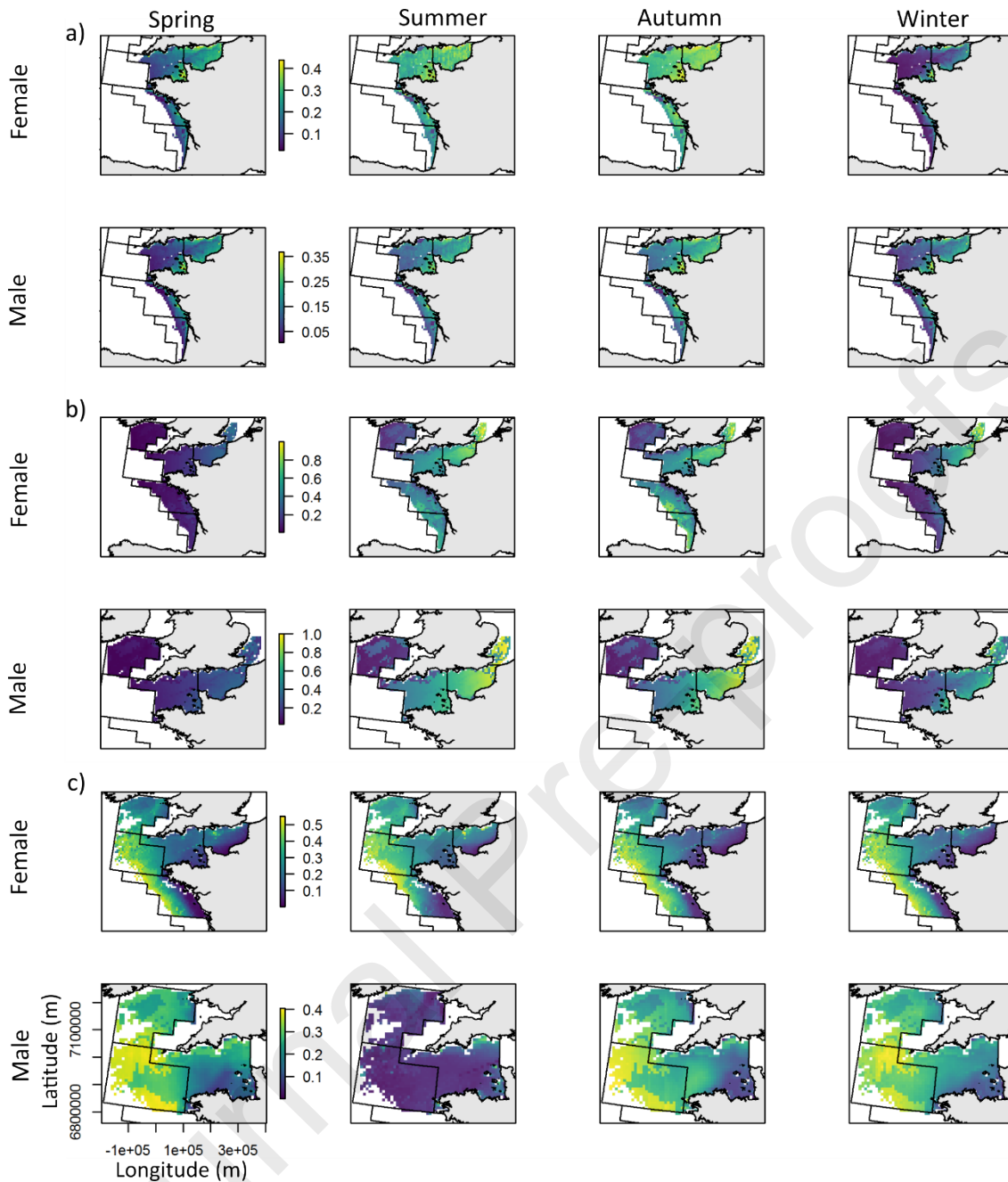
Fig. 5. Female and male a) Raja undulata b) Raja clavata c) Raja montagui predicted distribution maps (10 km 2 cells) per season. The legend represents the probability of presence. Black solid lines delineate ICES statistical divisions.
