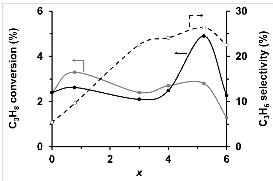
Figure 11. Influence of the substitution of phosphates by vanadates of \text{Ca}_{10}(\text{PO}_4)_{6-x}(\text{VO}_4)_x(\text{OH})_{2-y}\text{O}_y samples on \text{C}_3\text{H}_8 conversion ( \bullet ), \text{C}_3\text{H}_8 conversion normalized with respect to the specific surface area of the V-free sample ( \text{Ca}_{10}(\text{PO}_4)_6(\text{VO}_4)_0(\text{OH})_2 : 35 \text{ m}^2/\text{g} ) ( \bullet ) and \text{C}_3\text{H}_6 selectivity ( \circ ) (7.4% \text{C}_3\text{H}_8 , 2.2% \text{O}_2 in He, 12.5 \text{ mL}_{\text{NTP}} \text{ min}^{-1} total flow) at 723 K.
