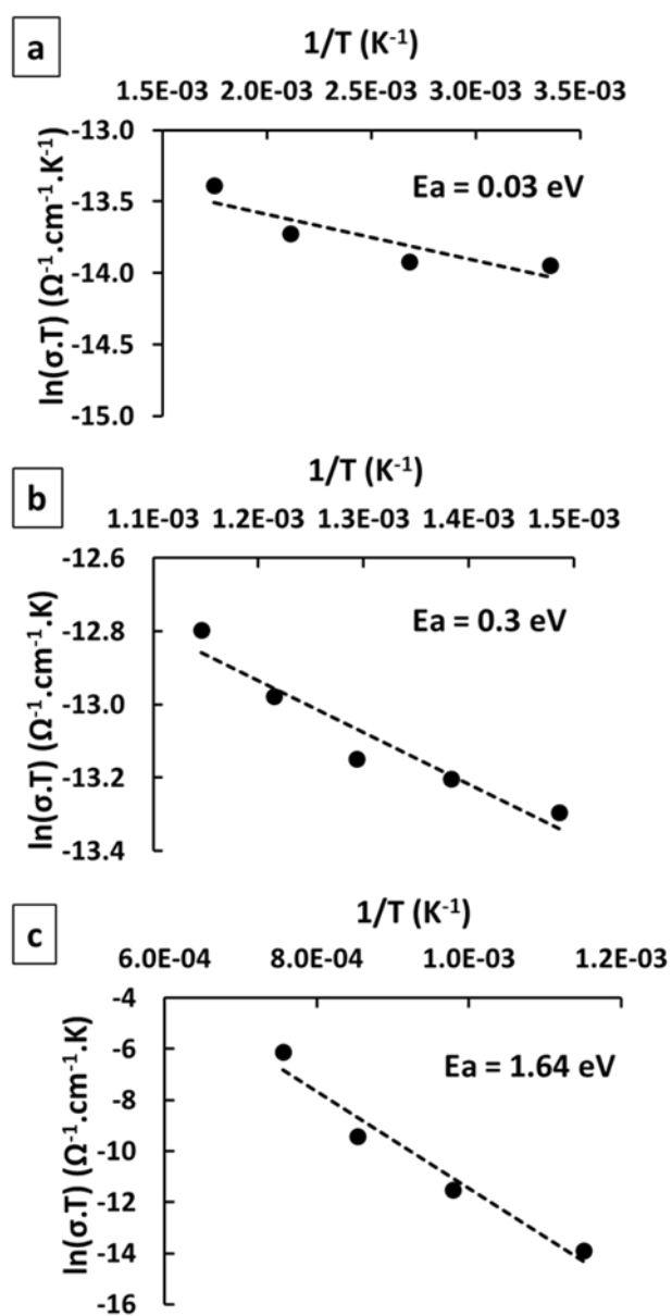
Figure S2: Arrhenius plots of the ionic conductivity of \text{Ca}_{10}(\text{PO}_4)_{0.78}(\text{VO}_4)_{5.22}(\text{OH})_{1.32}\text{O}_{0.34} for the a) low, b) intermediate and c) high temperature domains.
