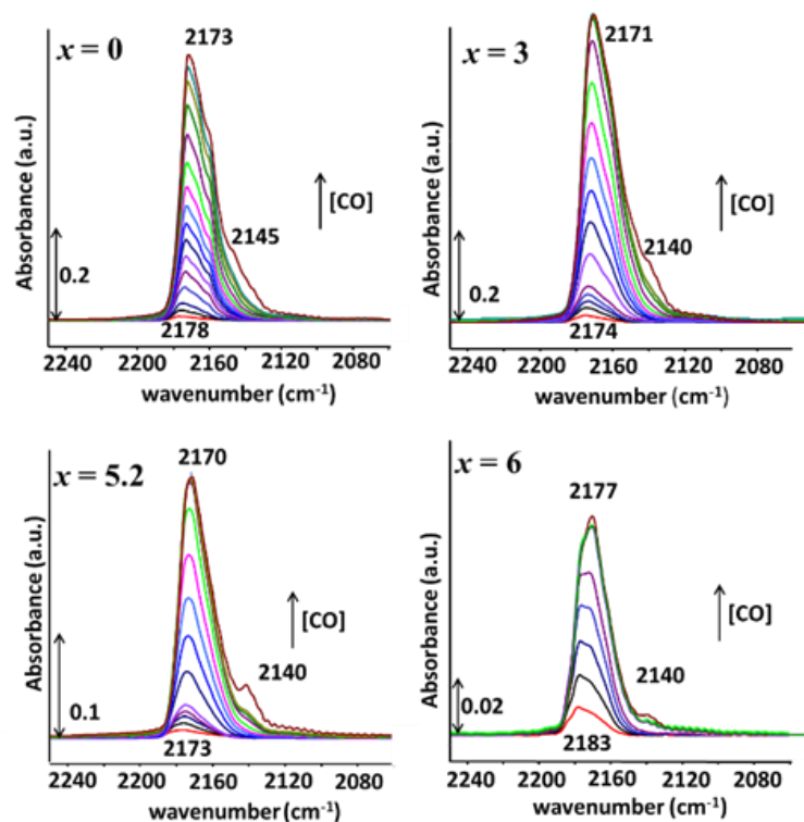
Figure 1. FTIR difference spectra in the 2230-2070 \text{cm}^{-1} region of self-supported wafers of \text{Ca}_{10}(\text{PO}_4)_6-x(\text{VO}_4)_x(\text{OH})_2 samples with x = 0, 3, 5.2 and 6 after adsorption of incremental doses of CO up to an equilibrium pressure of 133 Pa at 100 K
