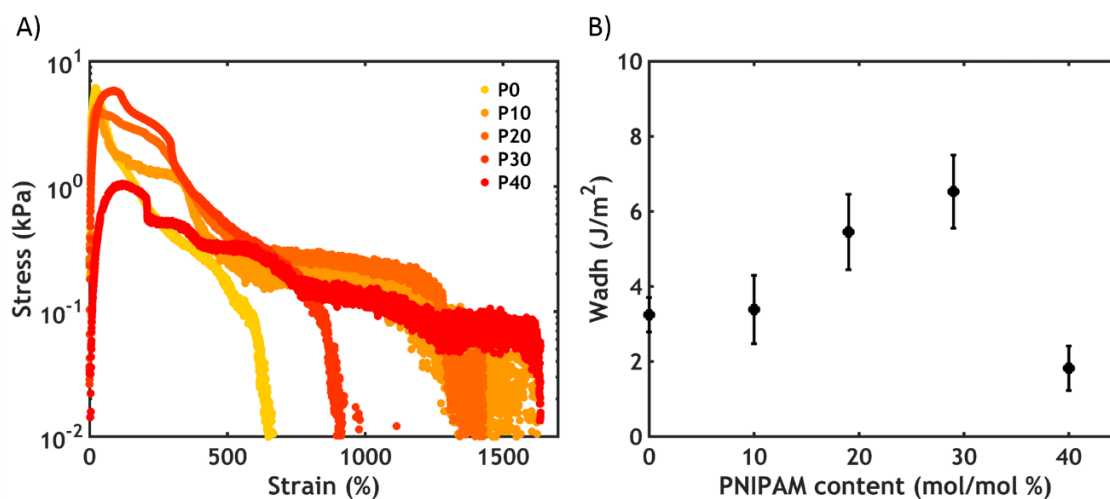
Figure 14. Underwater adhesion performance obtained after the salt-activated setting process for the samples P x S0.75. (A) Stress-strain curves plotted in log-lin scale and (B) work of adhesion as a function of the PNIPAM content.
