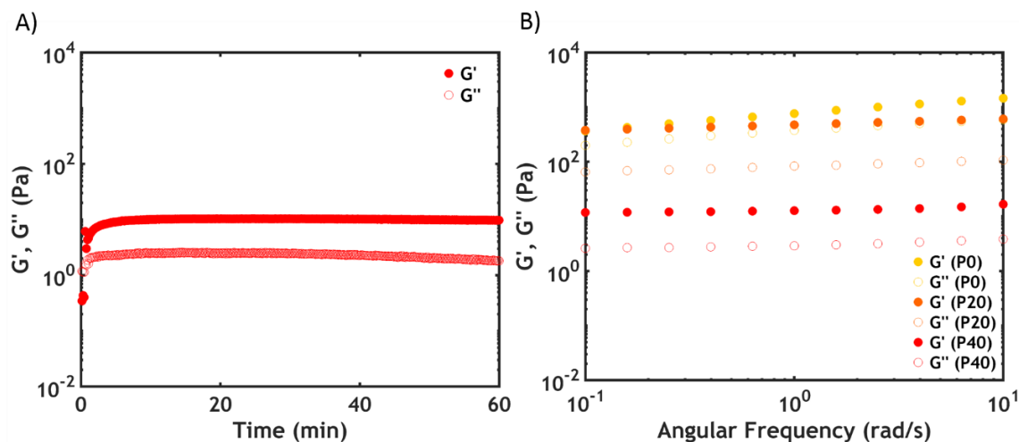
Figure 13. (A) Time sweeps performed on P40S0.75 and (B) frequency sweeps performed on samples P x S0.75 immediately after the salt-activation at 20 °C. Filled dots represent G' , while hollow dots represent G'' .
