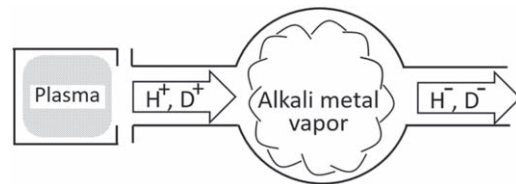
Figure 5. A schematic showing a double charge exchange type negative ion source.
