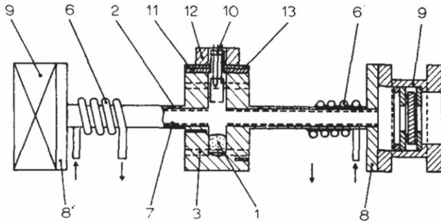
Figure 6. Vertical section of the cesium charge-exchange cell. 1: cesium reservoir; 2: charge-exchange canal; 3: heater; 6: copper coils brazed to the extremities of the cell; 7: wick; 8: flange; 9: slide-valve; 10: surface ionization gauge; 11: flange supporting the surface ionization gauge; 12: oven; 13: asbestos sheet. (Figure 1 of [75].) With permission from M Bacal et al 1974 Nucl. Instrum. Methods 114 407, ELSEVIER.
