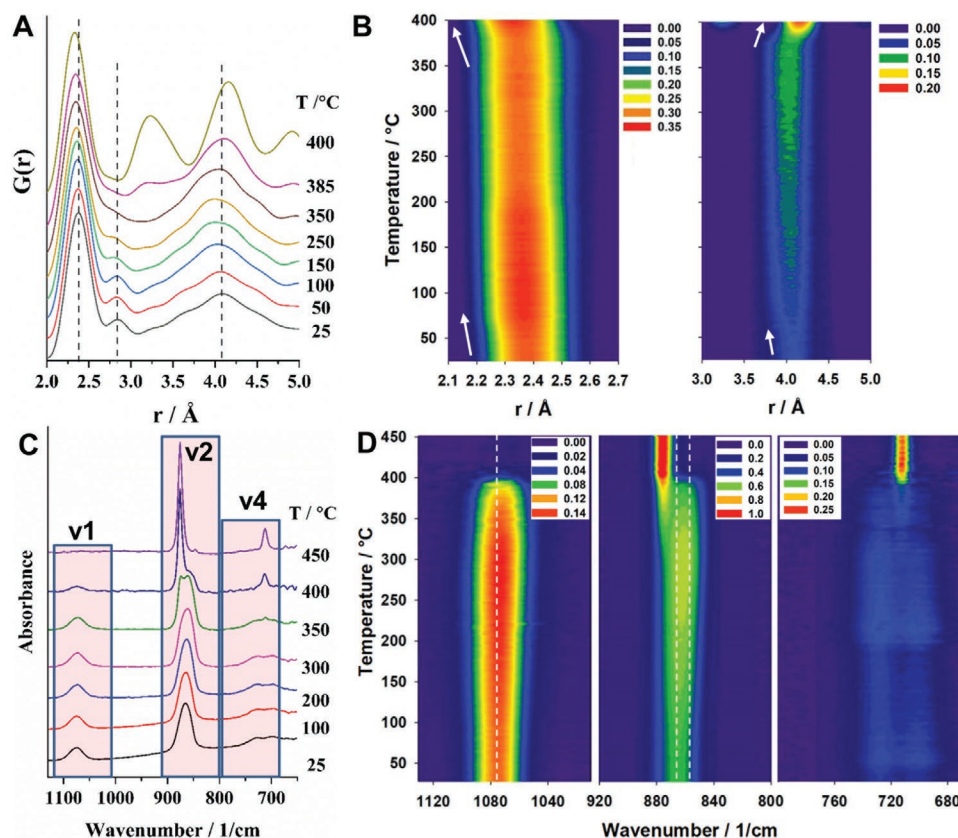
Figure 5. PDF patterns A) of ACC S -3% at different temperatures during in situ heating at 3 \text{ }^{\circ}\text{C min}^{-1} and corresponding contour plots B). White arrows indicate the shifts of the peaks. FTIR C) spectra of ACC S -3% at different temperatures during in situ heating at 3 \text{ }^{\circ}\text{C min}^{-1} and the corresponding contour plot D) of different bands after background subtraction. Black dashed lines in D) are used to better visualize the evolution of the peaks.
