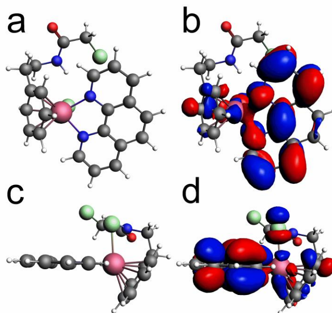
Fig. 3 Optimized chemical structure of 1 (a,c) and its SOMO orbital (b,d). Carbon atoms are shown in grey, nitrogen in blue, oxygen in red, chlorine in green and ruthenium in pink color, respectively.
