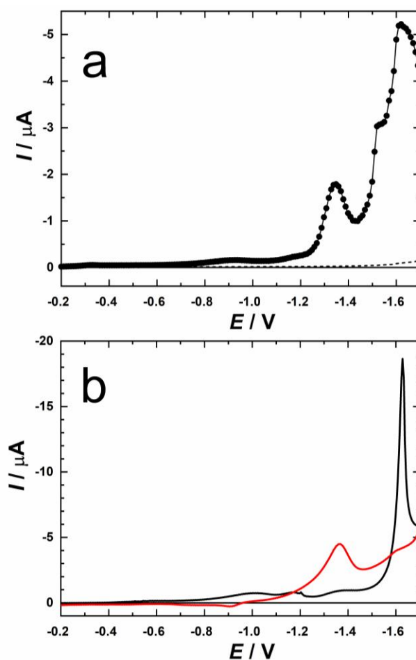
Fig. 4 DC polarography (a) and cyclic voltammetry (b) of 1.8 \times 10^{-5} M 1 in 0.1 M aqueous KCl solution on mercury electrode. DME drop time was 2 seconds (a) and HMDE scan rate was 0.5 V/s (b). Red line indicates the backward scan from -1.7 V to -0.2 V.
